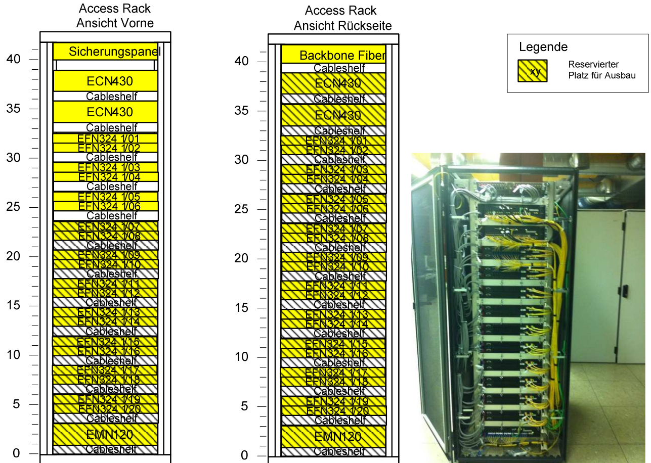
Abbildung 60 Racklayouts Access Knoten, FDA ewb Rack Front SBRE
